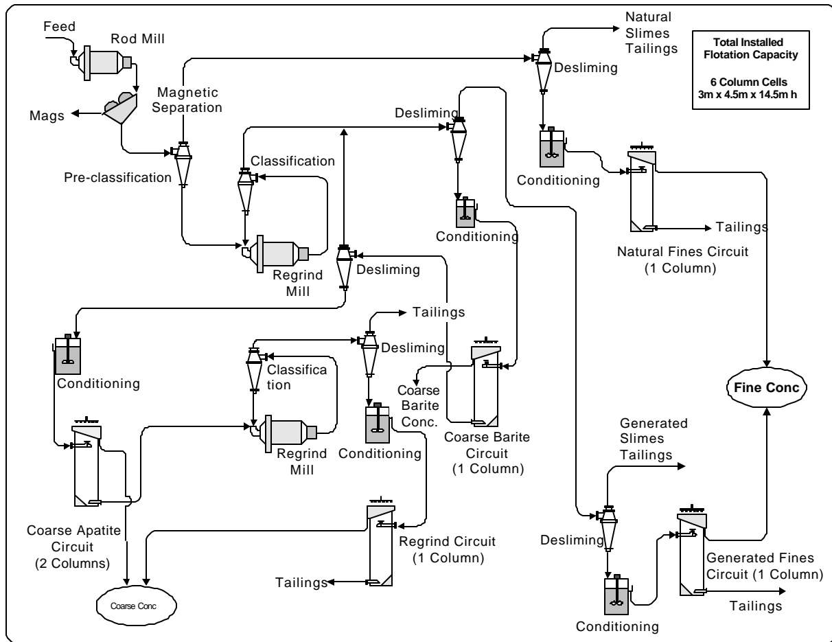
Figure 2 - Phosphate flotation circuit using CPT columns
